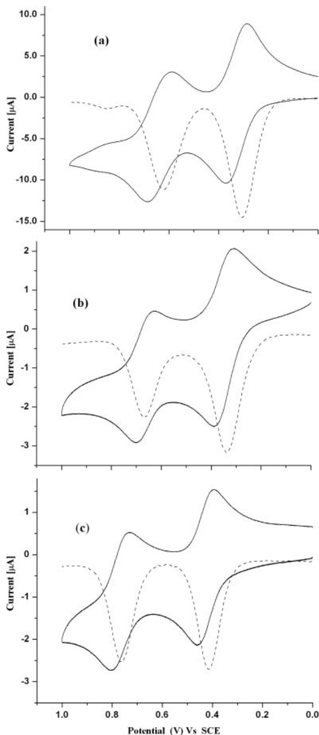
Figure 5. Cyclic voltammograms (solid line) and differential pulse voltammograms (dashed line) of (a) 6e , (b) 7a , and (c) 10 in \text{CH}_2\text{Cl}_2 containing 0.1 M \text{TBAPF}_6 , recorded at a scan speed of 100 \text{ mV s}^{-1} .
