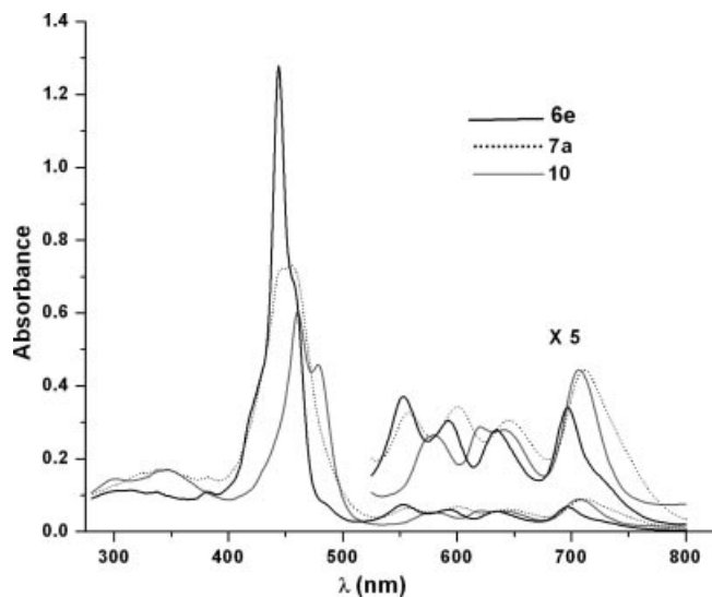
Figure 2. Electronic absorption spectra of 6e , 7a , and 10 in \text{CH}_2\text{Cl}_2 at a concentration of 0.5 \times 10^{-6} M.
