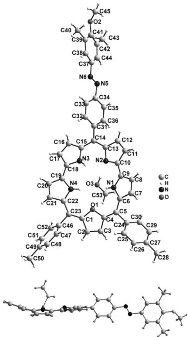
Figure 7. Single-crystal X-ray structure of 7a with one trapped methanol molecule: (a) top view; (b) side view ( meso -phenyl rings have been omitted for clarity; dotted lines show the hydrogen bond between methanol and the pyrrole NH groups).
