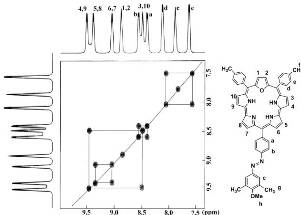
Figure 1. ^1\text{H} - ^1\text{H} COSY spectrum of 7a with assignments in the aromatic region.
