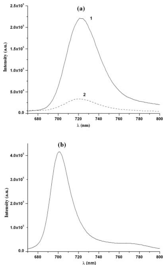
Figure 4. (a) Emission spectra of 7a (bold line: \lambda_{\text{exc}} = 444\text{ nm} ; dotted line: \lambda_{\text{exc}} = 325\text{ nm} ); (b) emission spectrum of 6e ( \lambda_{\text{exc}} = 444\text{ nm} ).
