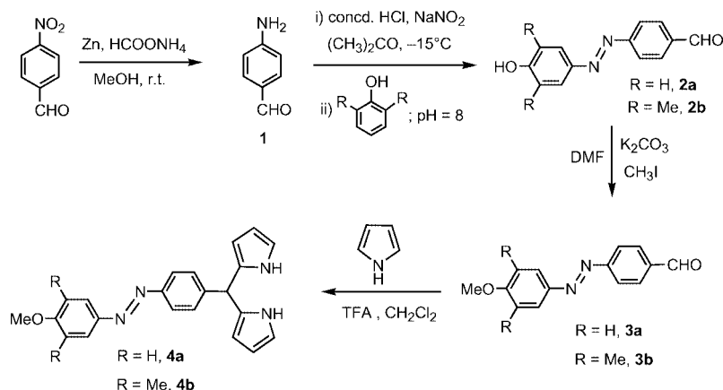
Scheme 1. Synthesis of dipyrromethanes 4a,b .
