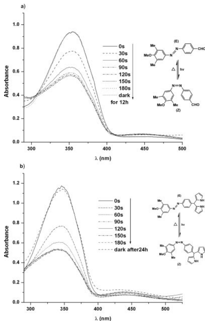
Figure 3. UV/Vis absorption spectral changes of the reversible ( E )/( Z ) isomerization of (a) 3b and (b) 4b in toluene. The irradiation time is shown in seconds.
