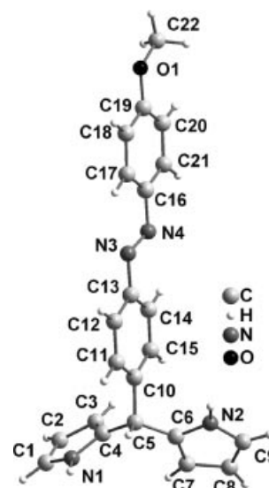
Figure 6. Single-crystal X-ray structure of 4a .
