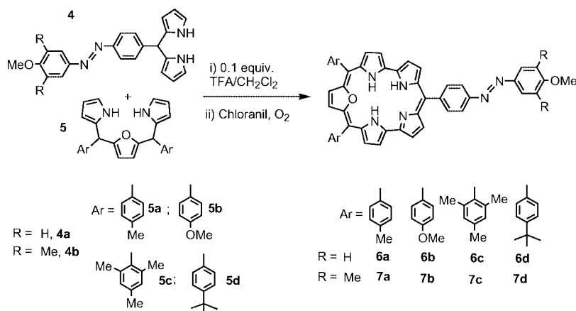
Scheme 2. Synthesis of azobenzene-smaragdyrin conjugates.
